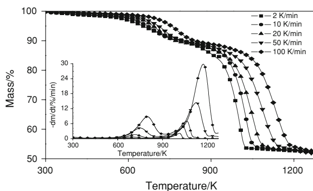
Fig. 1 TG curves of Oil Shale at different heating rates. Inset: corresponding DTG curves
