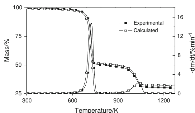
Fig. 6 Comparison between experimental and calculated TG/DTG values for the oil shale/PET mixture at 10 K/min
