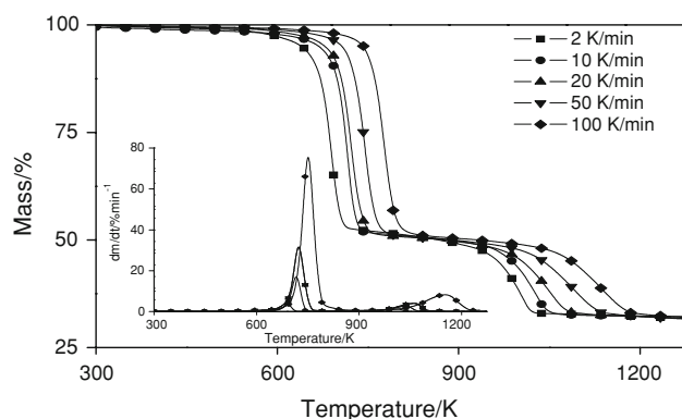
Fig. 5 TG curves of Oil shale/PET mixture at different heating rates. Inset: corresponding DTG curves
