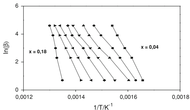
Fig. 2 Ozawa-Flynn-Wall plots for Oil Shale thermal degradation
