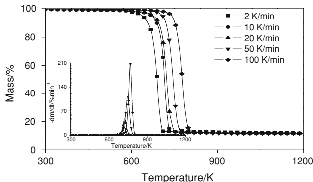
Fig. 3 TG curves of PET at different heating rates. Inset : corresponding DTG curves
