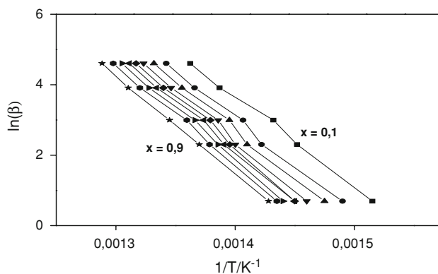
Fig. 4 Ozawa-Flynn-Wall plots for PET thermal degradation
