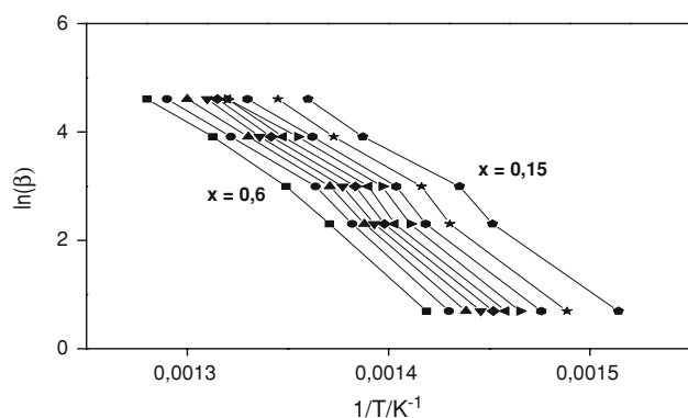
Fig. 7 Ozawa-Flynn-Wall plots for Oil shale/PET mixture thermal degradation
